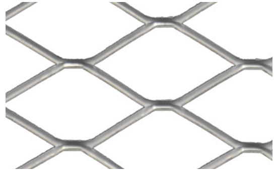
Masche Mesh freier Querschnitt ca. free cross-section approx. 62 x 23 x 3,0 x 2,5 [mm] 73,9%
