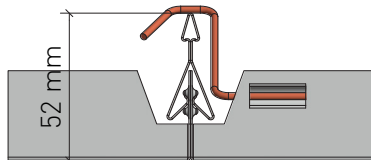
Detail A Detale A
