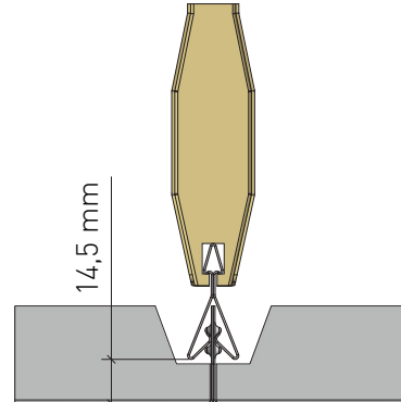
Detail B Detale B
