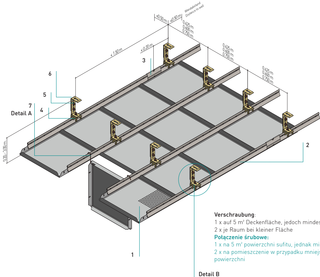
Detail B
