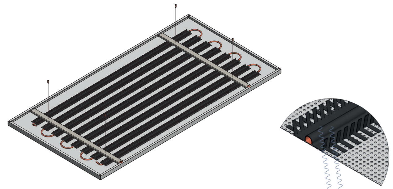
Innovative acoustic guide profile - ALP Sound waves are only partially reflected
