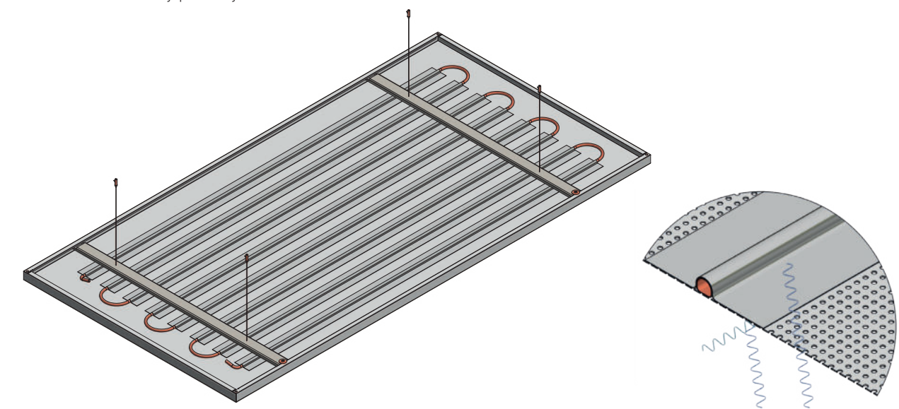
Conventional heat guiding plate Sound waves are completely reflected by the heat guiding plate
