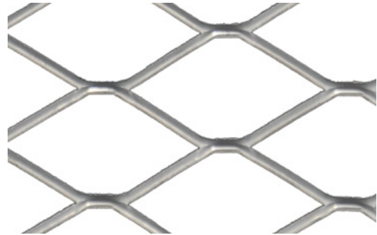
Masche Mesh freier Querschnitt ca. free cross-section approx. 62 x 23 x 3,0 x 2,5 [mm] 73,9%
