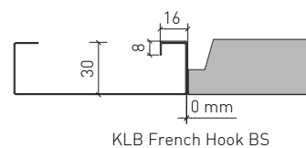
KLB French Hook BS
